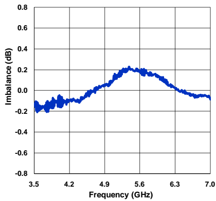
Amplitude Imbalance
