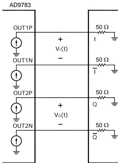
Figure 2. AD9783 Driving AM3570N
