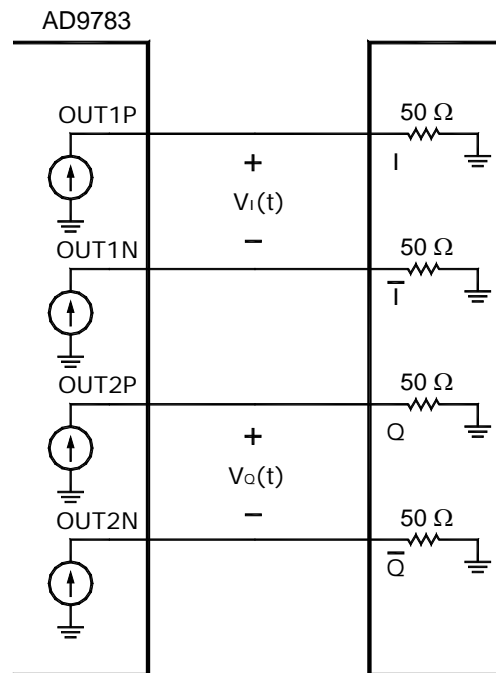
Figure 2. AD9783 Driving AM70100N
