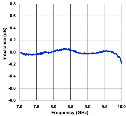
Amplitude Imbalance
