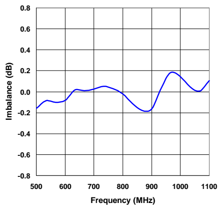
Amplitude Imbalance
