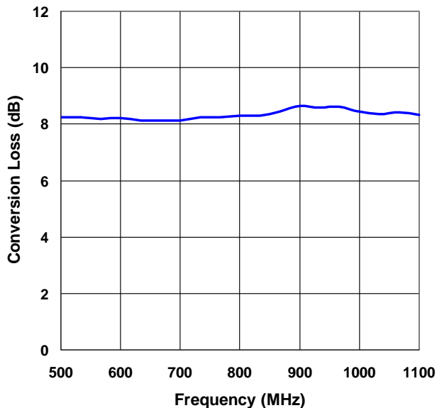
Conversion Loss
