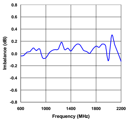
Amplitude Imbalance
