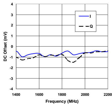
DC Offsets
