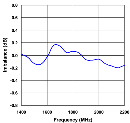
Amplitude Imbalance
