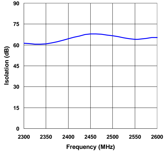
LO-RF Isolation
