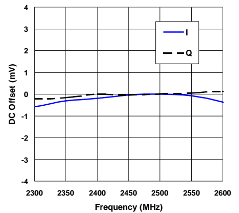
DC Offsets
