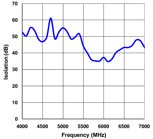
LO-RF Isolation
