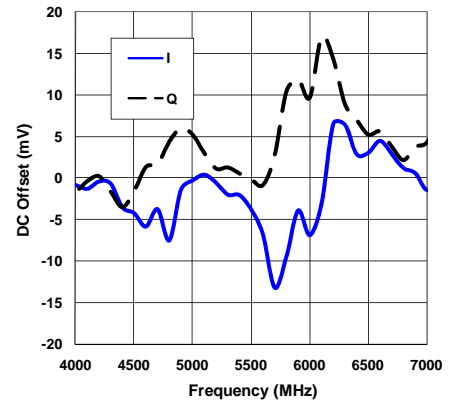
DC Offsets
