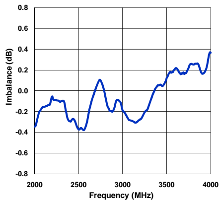
Amplitude Imbalance
